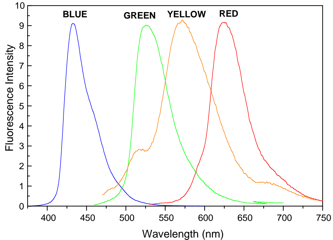
Normalized intensity for MME FluorRef Slides (FluorRefs invented by Dr. P. C. Cheng; Spectra courtesy of H. Malak, Microcosm)
