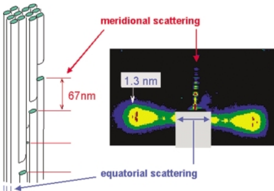
Figure 7 Small-angle X-ray scatter (SAXS) spectrum of polymer fibrils. (Image courtesy of Bruker-AXS.)
