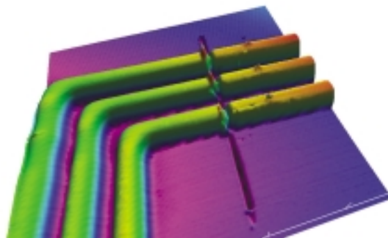
Figure 5 MEMS device showing both a nanoscratch test (middle) and nanoindentation tests for nanohardness. (Image courtesy of Hysitron .)
